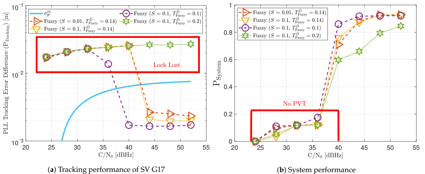
Figure 30. Dynamic performance of FL at different C/N_0 levels.
