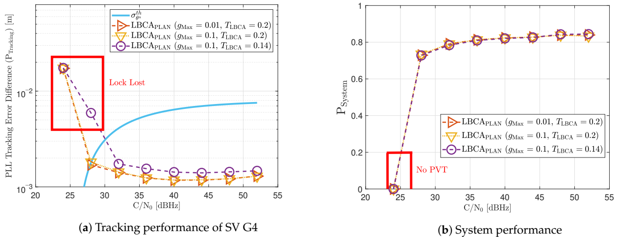
(a) Tracking performance of SV G4 (b) System performance Figure 25. Static performance of LBCA PLL with PLAN interpolation at different C/N_0 levels.
