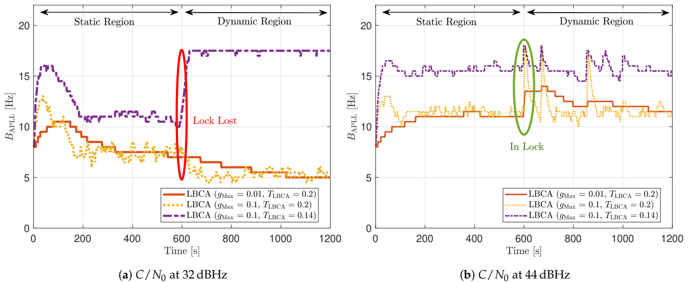
(a) C/N_0 at 32 dBHz (b) C/N_0 at 44 dBHz Figure 33. PLL loop bandwidth update with LBCA of SV G17 tracking in dynamic scenario.
