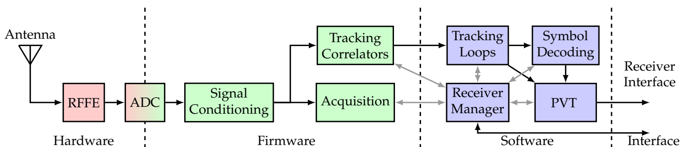
Figure 14. GOOSE architecture diagram.
