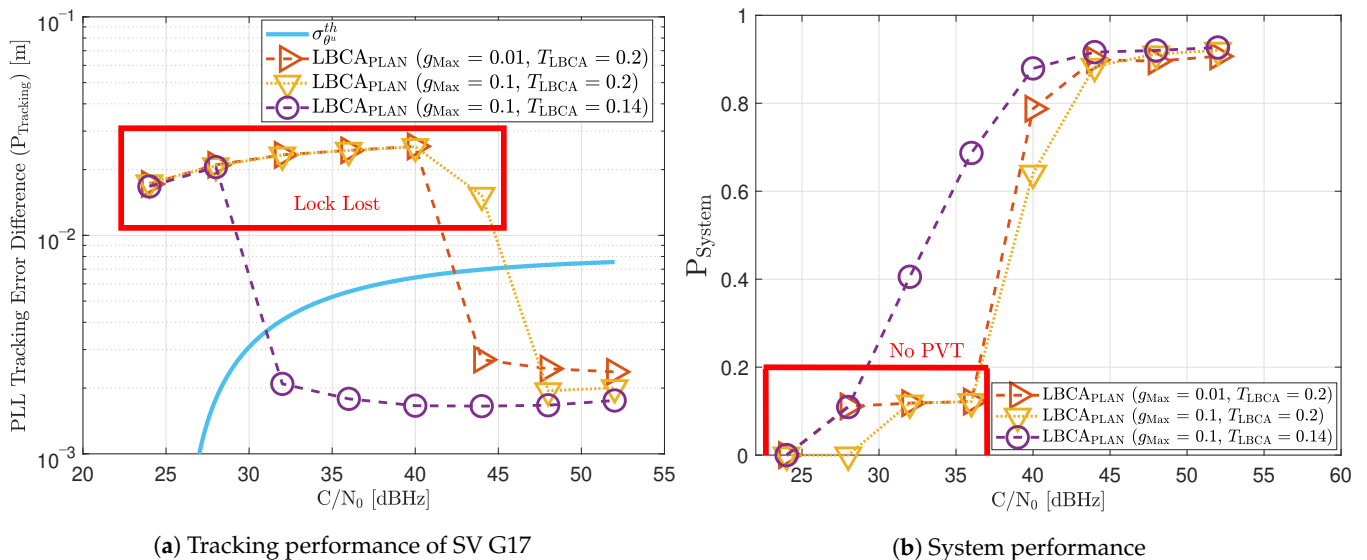
Figure 34. Dynamic performance of LBCA with PLAN interpolation at different C/N_0 levels.
