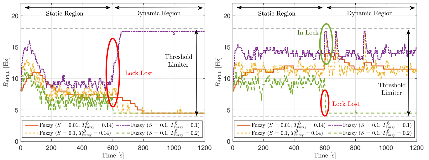
(a) C/N_0 at 32 dBHz (b) C/N_0 at 44 dBHz Figure 31. PLL loop bandwidth update with FL of SV G17 tracking in dynamic scenario.
