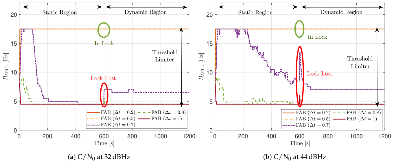
Figure 29. PLL loop bandwidth update with FAB of SV G17 tracking in dynamic scenario.
